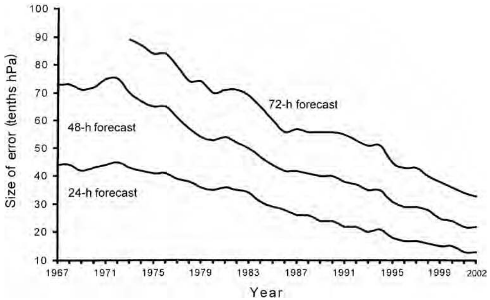
Figure 5.5 Errors (root mean square differences of forecasts of surface pressure compared with analyses) of UK Meteorological Office forecasting models for the north Atlantic and Western Europe since 1966 for 24-h, 48-h and 72-h forecasts. Note that 1 hPa = 1 mbar.
