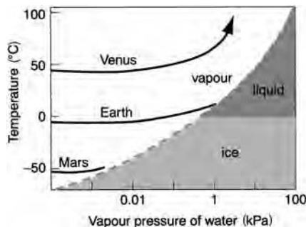
Figure 2.7 Illustrating the evolution of the atmospheres of the Earth, Mars and Venus. In this diagram, the surface temperatures of the three planets are plotted against the vapour pressure of water in their atmospheres as they evolved. Also on the diagram (dashed) are the phase lines for water, dividing the diagram into regions where vapour, liquid water or ice are in equilibrium. For Mars and the Earth the greenhouse effect is halted when water vapour is in equilibrium with ice or liquid water. For Venus no such halting occurs and the diagram illustrates the 'runaway' greenhouse effect.
