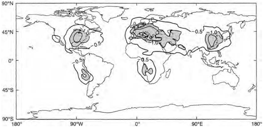
Figure 3.7 Modelled geographic distribution of estimates of the annual mean direct radiative forcing (in watts per square metre) from anthropogenic sulphate aerosols in the troposphere. The radiative forcing, which is negative, is largest in regions close to industrial activity.
