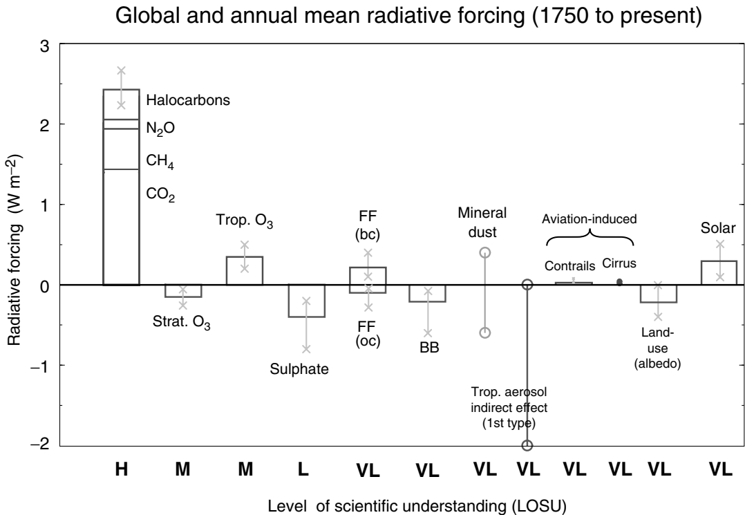
Figure 3.8 Global, annual mean radiative forcings ( \text{W m}^{-2} ) due to a number of agents for the period from pre-industrial (1750) to 2000. The height of the rectangular bar denotes a best estimate value while its absence denotes no best estimate is possible because of large uncertainties. The vertical lines with 'x' or 'o' delimiters indicates estimates of the uncertainty ranges. A 'level of scientific understanding (LOSU)' index is accorded to each forcing, with H, M, L and VL denoting high, medium, low and very low levels respectively. This represents a judgement about the reliability of the forcing estimate involving factors such as the assumptions necessary to evaluate the forcing, the degree of knowledge of the mechanisms determining the forcing and the uncertainties surrounding the quantitative estimate of the forcing. The well-mixed greenhouse gases are grouped together into a single rectangular bar with the individual contributions shown. The second and third bars apply to stratospheric and tropospheric ozone. The next bars denote the direct effect of aerosols. FF denotes aerosol from fossil fuel burning and is separated into black carbon (bc) and organic carbon (oc) components. BB denotes aerosols from biomass burning. The sign of the effects due to mineral dust is itself an uncertainty. Only the first indirect aerosol effect is estimated as little quantitative evidence exists regarding the second. All the forcings have distinct spatial and seasonal variations (see Figure 3.7) so that they cannot be added up and viewed a priori as providing offsets in terms of complete global climate impact.
