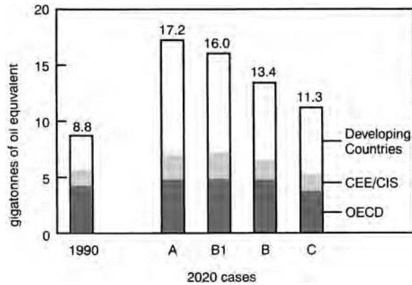
Figure 11.5 Primary energy demand by economic groupings of countries for WEC scenarios.
