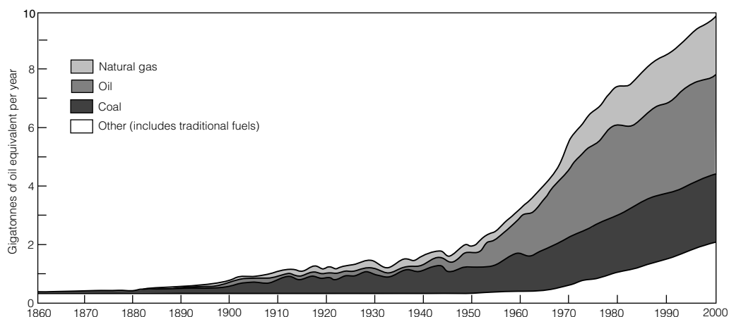
Figure 11.1 Growth in the rate of energy use and in the sources of energy since 1860 in thousand millions of tonnes of oil equivalent (Gtoe) per year. In terms of primary energy units, 1 Gtoe = 41.87 exajoules (1 exajoule (EJ) = 10^{18} J). Of the 'other' in 2000, approximately 0.9 Gtoe is attributed to traditional fuels, 0.7 Gtoe to nuclear energy and 0.6 Gtoe to hydro and other renewables (source: Report of G8 Renewable Energy task Force, July 2001).
