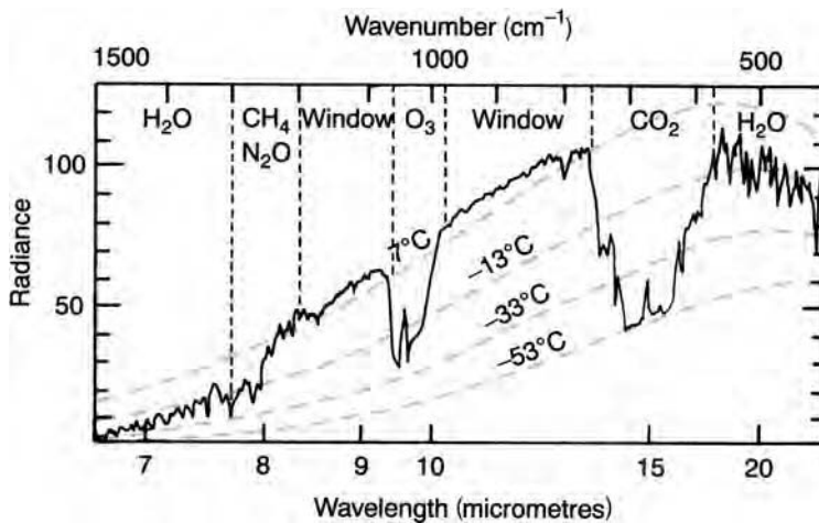
Figure 2.4 Thermal radiation in the infrared region (the visible part of the spectrum is between about 0.4 and 0.7\ \mu\text{m} ) emitted from the Earth's surface and atmosphere as observed over the Mediterranean Sea from a satellite instrument orbiting above the atmosphere, showing parts of the spectrum where different gases contribute to the radiation. Between the wavelengths of about 8 and 14\ \mu\text{m} , apart from the ozone band, the atmosphere, in the absence of clouds, is substantially transparent; this is part of the spectrum called a 'window' region. Superimposed on the spectrum are curves of radiation from a black body at 7^{\circ}\text{C} , -13^{\circ}\text{C} , -33^{\circ}\text{C} and -53^{\circ}\text{C} . The units of radiance are watts per square metre per steradian per wavenumber.
