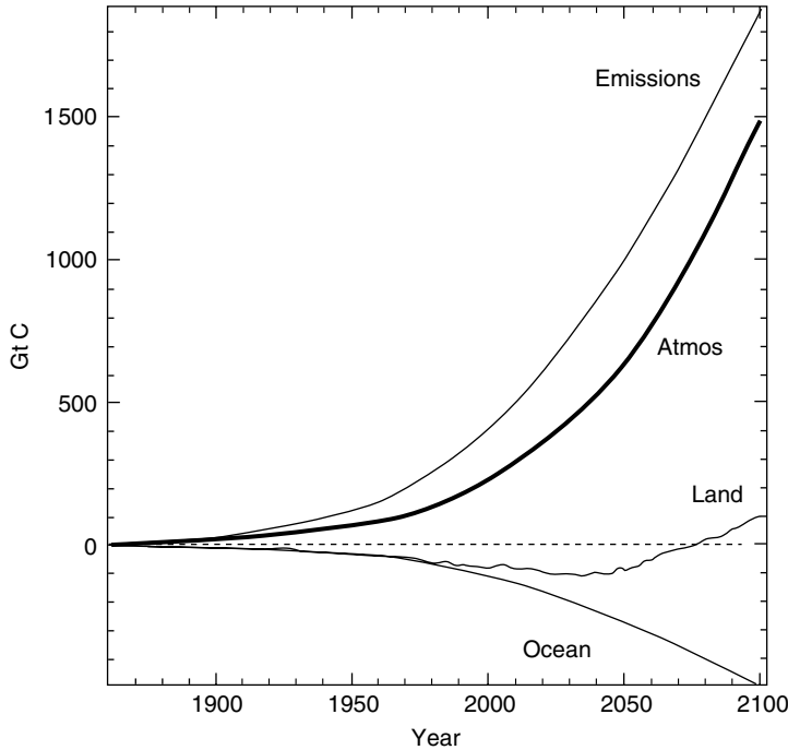
Figure 3.5 Illustrating the possible effects of climate feedbacks on the carbon cycle. Results are shown of the changing budgets of carbon (in gigatonnes of carbon) in the atmosphere, land and ocean in an ocean–atmosphere model coupled to an ocean carbon cycle model (which includes the transfer of carbon dioxide to depth through both the solubility pump and the biological pump) and a dynamic global vegetation model (which includes the exchange of carbon with the soil and with five different types of plant). The model was run with the fossil fuel carbon dioxide emissions from 1860 to the present and then projected to 2100 assuming the IS 92a scenario shown in Figure 6.1. Note that because of climate feedbacks, the terrestrial biosphere changes from being a net sink of carbon to being a net source around the middle of the twenty-first century. Note also as this source becomes stronger, by 2100 the atmospheric carbon content is increasing at about the same rate as the total emissions (i.e. the ‘airborne fraction’, or the fraction of fossil fuel emissions that remains in the atmosphere, has changed from being about a half in the year 2000 to being about unity in 2100). Note also that an atmospheric carbon content of 1500 Gt more than it was in 1860 is equivalent to a concentration of nearly 1000 ppm.
