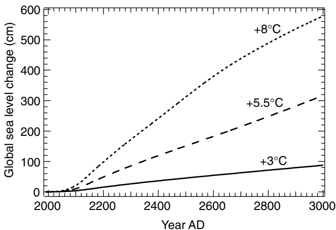
Figure 7.3 Global average sea level changes due to the response of the Greenland ice-sheet to three climate warming scenarios during the third millennium. The labels on the curves refer to the mean annual temperature rise over Greenland by 3000 AD as predicted by a two-dimensional climate and ocean model forced by greenhouse gas concentration rises until 2130 and kept constant after that. Note that projected temperature rises over Greenland are generally greater than those for global averages (by a factor of 1.2 to 3.1 for the AOGCMs used in generating Figure 6.4).
