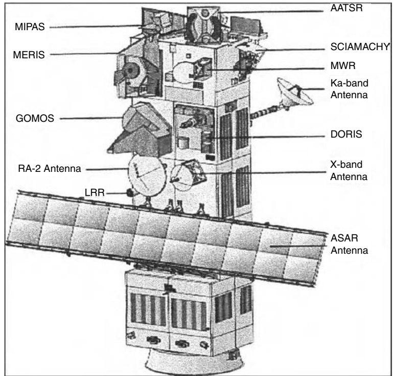
Figure 9.2 ENVISAT showing the instruments included in its payload: the Advanced Along-Track Scanning Radiometer (AATSR), the Michelson Interferometer for Passive Atmospheric Sounding (MIPAS), the Medium Resolution Imaging Spectrometer (MERIS), the SCanning Image Absorption spectroMeter for Atmospheric CartographY (SCIAMACHY), the MicroWave Radiometer (MWR), the Global Ozone Monitoring by Observation of Stars (GOMOS), the Radar Altimeter – second generation (RA-2), the Advanced Synthetic Aperture Radar (ASAR), and other instruments for communication and exact tracking. DORIS stands for Doppler Orbitography and Radiopositioning Integrated by Satellite. In its 800-km Sun-synchronous orbit with the solar array deployed, it measures 26\text{ m} \times 10\text{ m} \times 5\text{ m} and weighs 8.1 tonnes.
