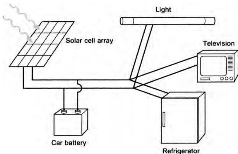
Figure 11.14 A simple 'solar home system' now being marketed in many countries in Africa, Asia and South America for a cost of a few hundred US$. An array of thirty-six solar cells, covering an area of 60 cm × 60 cm, provides around 40 W of peak power. This is sufficient to charge a car battery that can power up to three 9-W fluorescent lights and three hours of radio and one hour of television per day. With more restricted use of these devices or with a larger solar array, a small refrigerator can be added to the system.
