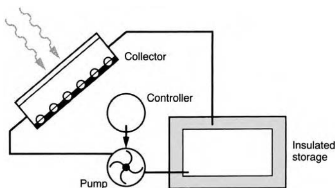
Figure 11.11 Design of a solar water heater: a solar collector connected to a storage tank through a circulating pump. Alternatively, if the storage is above the collector, the hot water will collect through gravity flow.
