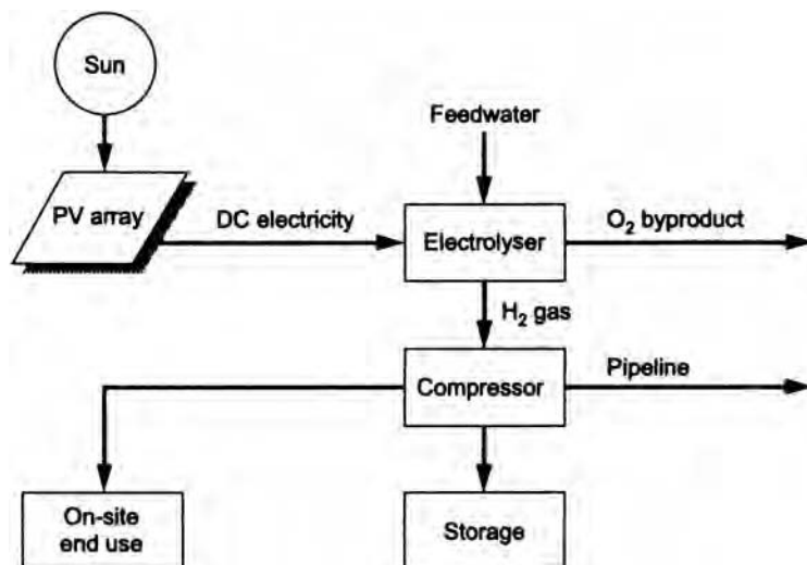
Figure 11.16 A solar photovoltaic (PV) electrolytic hydrogen system.
