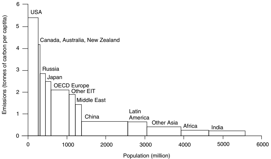
Figure 10.2 Carbon dioxide emissions in 2000 from different countries or groups of countries expressed per capita and population.
