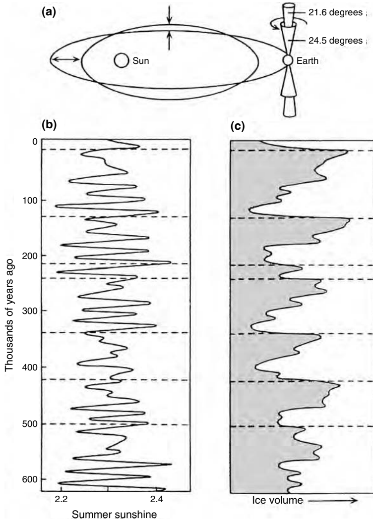
Figure 4.5 Variations in the Earth's orbit (a), in its eccentricity, the orientation of its spin axis (between 21.6^\circ and 24.5^\circ ) and the longitude of perihelion (i.e. the time of year when the Earth is closest to the Sun, see also Figure 5.19), cause changes in the average amount of summer sunshine (in millions of joules per square metre per day) near the poles (b). These changes appear as cycles in the climate record in terms of the volume of ice in the ice caps (c).
