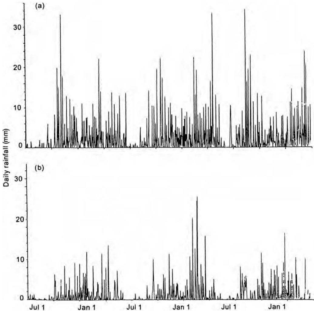
Figure 6.9 Daily rainfall for Italy for a three-year period simulated by a climate model, (a) for the current climate situation and (b) for the climate if the equivalent carbon dioxide concentration increased by a factor of four from its pre-industrial value (predicted for instance to occur before 2100 under the A2 scenario).
