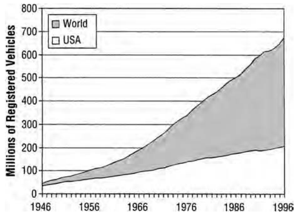
Figure 11.9 Growth of world motor vehicle population, 1946–96.
