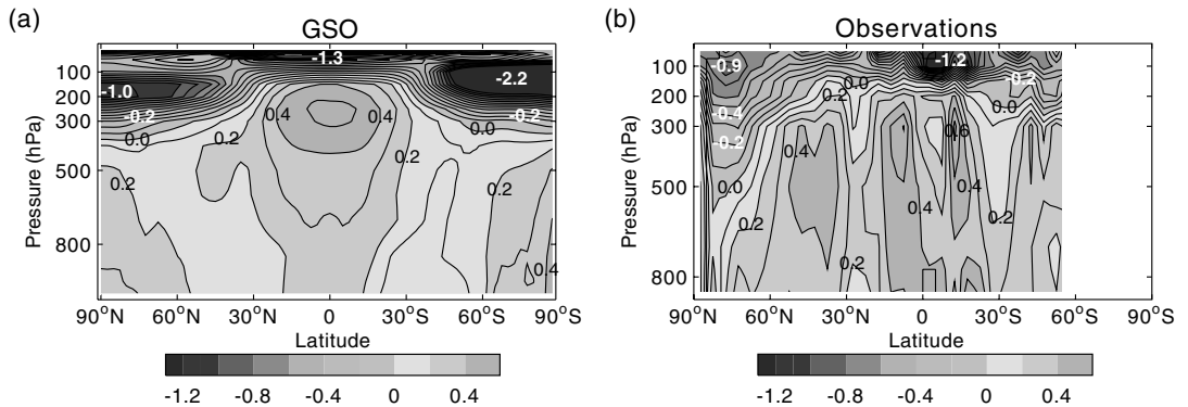
Figure 5.23 Simulated and observed zonal mean temperature change as a function of latitude and height. The changes plotted are the differences between the 1986–1995 decadal average and the twenty-year average from 1961 to 1980. The contour interval is 0.1^{\circ}\text{C} . (a) simulated changes taking into account increases in carbon dioxide, sulphate aerosols and the effect of observed changes in stratospheric ozone; (b) observed changes. A common pattern of stratospheric cooling and tropospheric warming is evident in the observations and both model experiments; the stratospheric cooling is partially due to the increase of carbon dioxide (see also Figure 4.2(b)) and the reduction in ozone (see Chapter 3).
