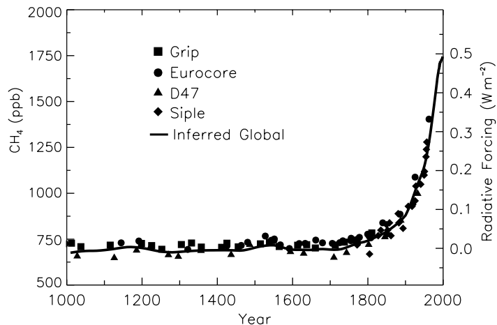
Figure 3.6 Change in methane concentration (mole fraction in ppb) over the last 1000 years determined from ice cores, glacier ice and whole air samples. Radiative forcing since the pre-industrial era due to the methane increase is plotted on the right axis.
