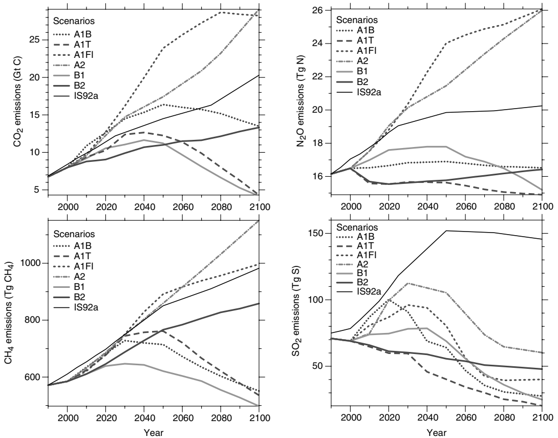
Figure 6.1 Anthropogenic emissions of carbon dioxide, methane, nitrous oxide and sulphur dioxide for the six illustrative SRES scenarios, A1B, A2, B1 and B2, A1FI and A1T. For comparison the IS 92a scenario is also shown.
