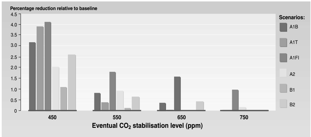
Figure 9.4 Global average GDP reduction in 2050 (relative to the baseline scenarios) for alternative stabilisation targets (see Chapter 10) and six SRES scenarios as baselines.
