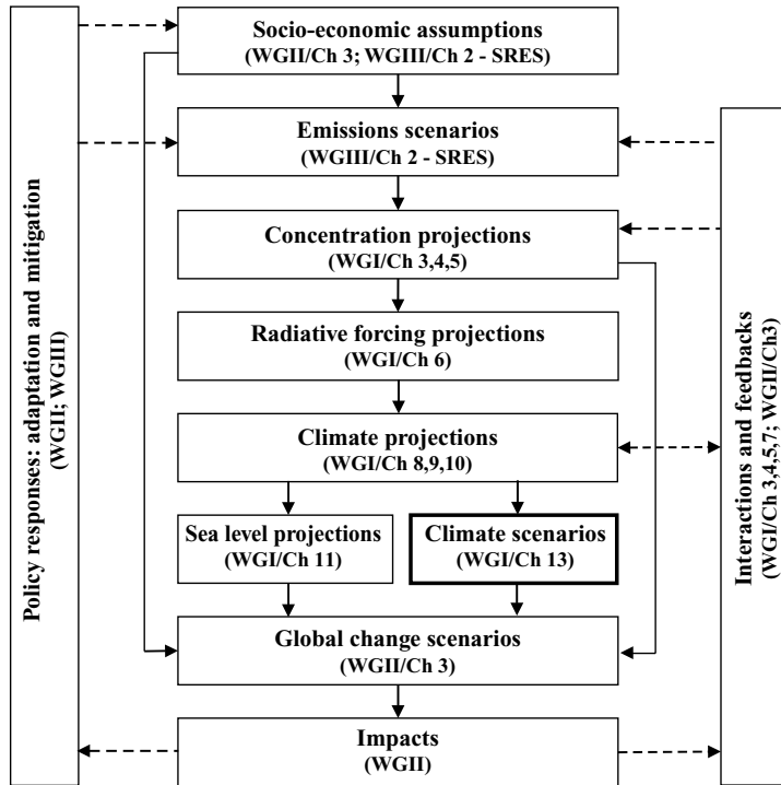
Figure 9.1 The cascade of uncertainties in projections to be considered in developing climate and related scenarios for climate change impact, adaptation and mitigation assessment. The chapters in the IPCC 2001 Report that deal with the various components are also identified.
