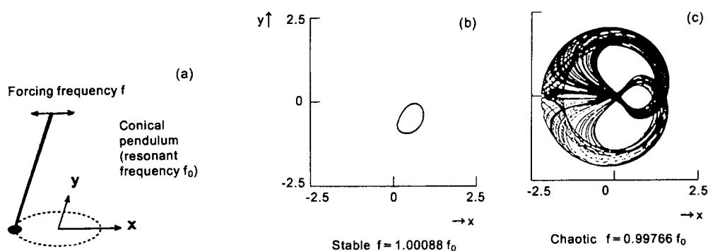
Figure 5.7 (a) Illustrating a simple pendulum consisting of a bob at the end of a string of length 10 cm attached to a point of suspension which is moved with a linear oscillatory forcing motion at frequencies near the pendulum's resonance frequency f_0 . (b) and (c) show plots of the bob's motion on a horizontal plane, the scale being in centimetres. (b) For a forcing frequency just above f_0 the motion of the bob settles down to a simple, regular pattern. (c) For a forcing frequency just below f_0 the bob shows 'chaotic' motion (although contained within a given region) which varies randomly and discontinuously as a function of the initial conditions.
