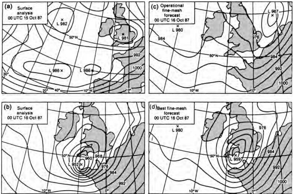
Figure 5.8 Analyses and forecasts of the surface pressure in millibars (1 mbar = 100 Pa = 1 hPa) for the storm which passed over southern England on 15/16 October 1987. The fully developed storm is shown in (b) about 4 hours before it reached the London area; (a) is the situation twenty-four hours earlier from which the storm developed. (c) and (d) are twenty-four-hour forecasts with the Meteorological Office operational fine-mesh model, (c) being the one available at the time and (d) being one produced after the event using more complete data and better assimilation procedures.
