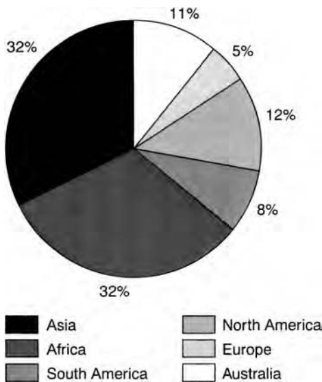
Figure 7.9 The world's drylands, by continent. The total area of drylands is about sixty million square kilometres (about forty per cent of the total land area), of which ten million are hyper-arid deserts.
