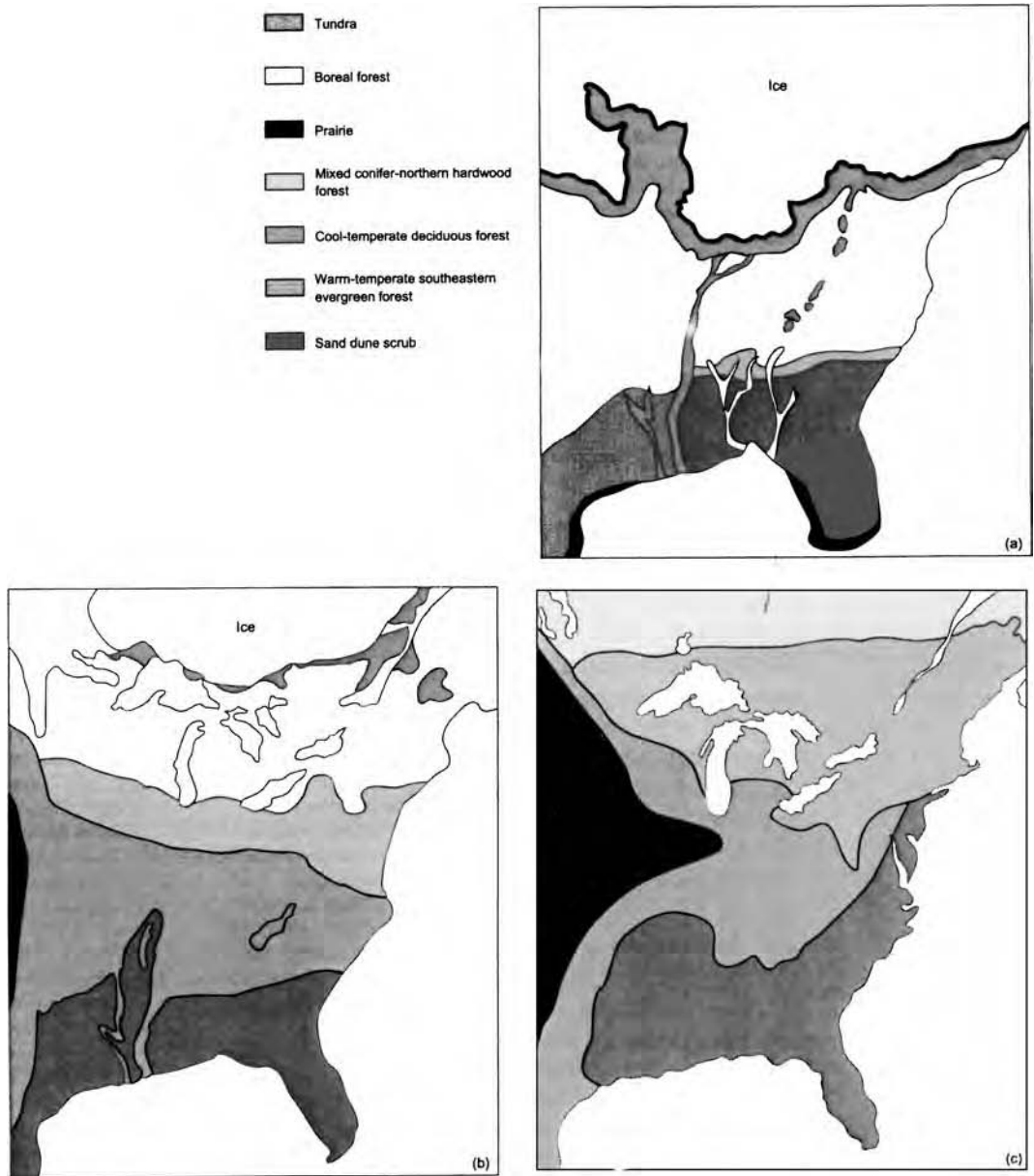
Figure 7.11 Vegetation maps of the south-eastern United States during past climate regimes: (a) for 18 000 years ago at the maximum extent of the last ice age, (b) for 10 000 years ago, (c) for 5000 years ago when conditions were similar to present. A vegetation map for 200 years ago is similar to that in (c).
