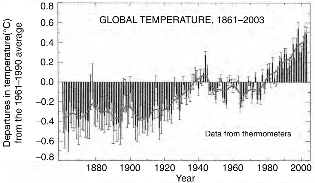
Figure 4.1 Variations of the globally averaged Earth's surface temperature over the last 140 years. The dark bars are the year by year averaged values; the grey line is a smoothed annual curve to illustrate decadal variations. Uncertainties in the data are also shown; the thin whiskers represent the 95% confidence range. The graph is based on an improved analysis of all years since the original publication in the Third IPCC Scientific Assessment. The changes are small.
