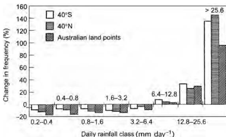
Figure 6.7 Changes in the frequency of occurrence of different daily rainfall amounts with doubled carbon dioxide as estimated by a CSIRO model in Australia.
