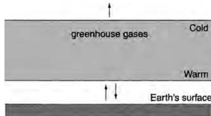
Figure 2.5 The blanketing effect of greenhouse gases.
