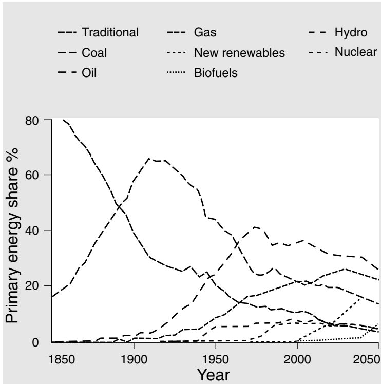
Figure 11.7 Energy transitions over two centuries. Under 'dynamics as usual' energy supplies continue to evolve from high to low carbon fuels and towards electricity as the dominant energy carrier – from increasingly distributed sources – driven by demands for security, cleanliness and sustainability.
