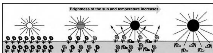
Figure 8.1 Daisyworld.
