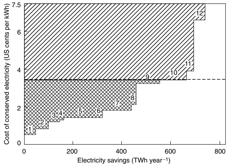
Figure 11.8 Cost of various options (at 1989 prices) for saving electricity in buildings. If the cost of conservation is less than the cost of the electricity saved over the lifetime of the application, a net saving results. The various options are: (1) use of white surfaces to reduce the need for air conditioning; (2) residential lighting; (3) residential water heating; (4) commercial water heating; (5) commercial lighting; (6) commercial cooking; (7) commercial cooling; (8) commercial refrigeration; (9) residential appliances; (10) residential space heating; (11) commercial and industrial space heating; (12) commercial ventilation. The shaded areas are all below 7.5 cents per kWh (the all-sector average electricity price) and 3.5 cents per kWh (typical operating cost of US electricity generation). The total savings in the figure add up to about forty-five per cent of the electricity use.
