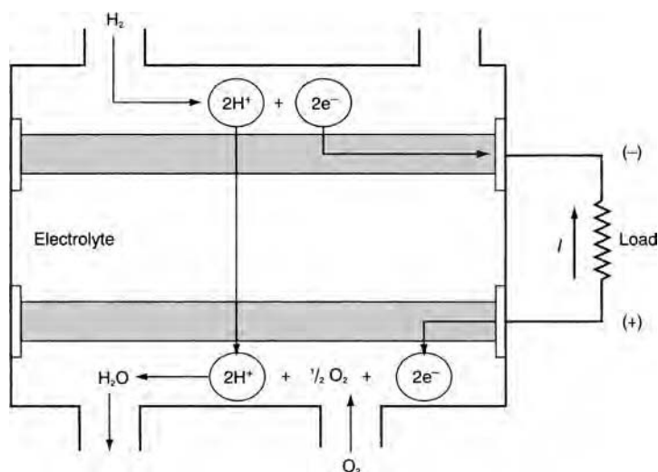
Figure 11.15 Schematic of a hydrogen-oxygen fuel cell. Hydrogen is supplied to the porous anode (negative electrode) where it dissociates into hydrogen ions ( H^+ ) and electrons. The H^+ ions migrate through the electrolyte (typically an acid) to the cathode (positive electrode) where they combine with electrons (supplied through the external electrical circuit) and oxygen to form water.
