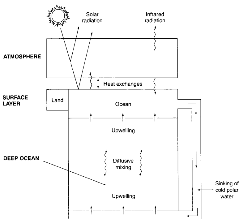
Figure 6.3 The components of a simple 'upwelling-diffusion' climate model.
