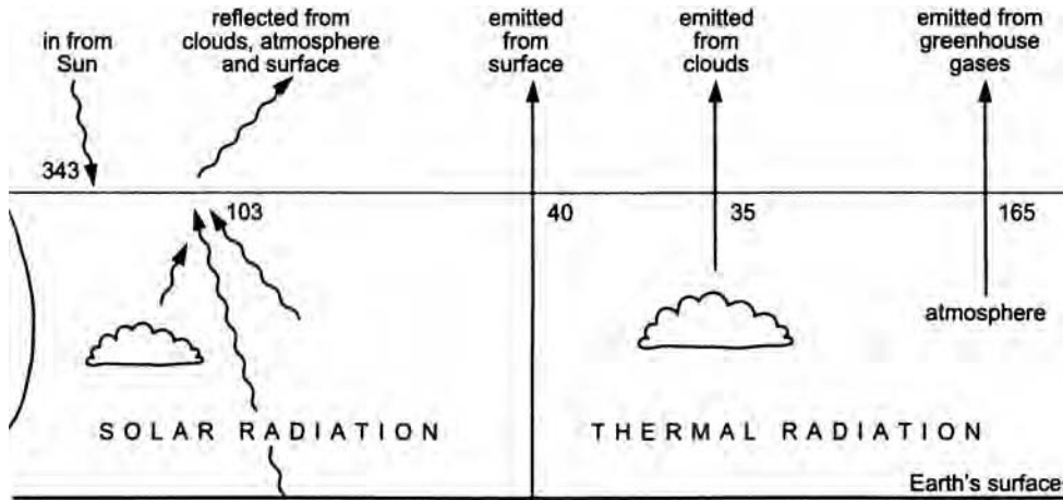
Figure 2.6 Components of the radiation (in watts per square metre) which on average enter and leave the Earth's atmosphere and make up the radiation budget for the atmosphere.
