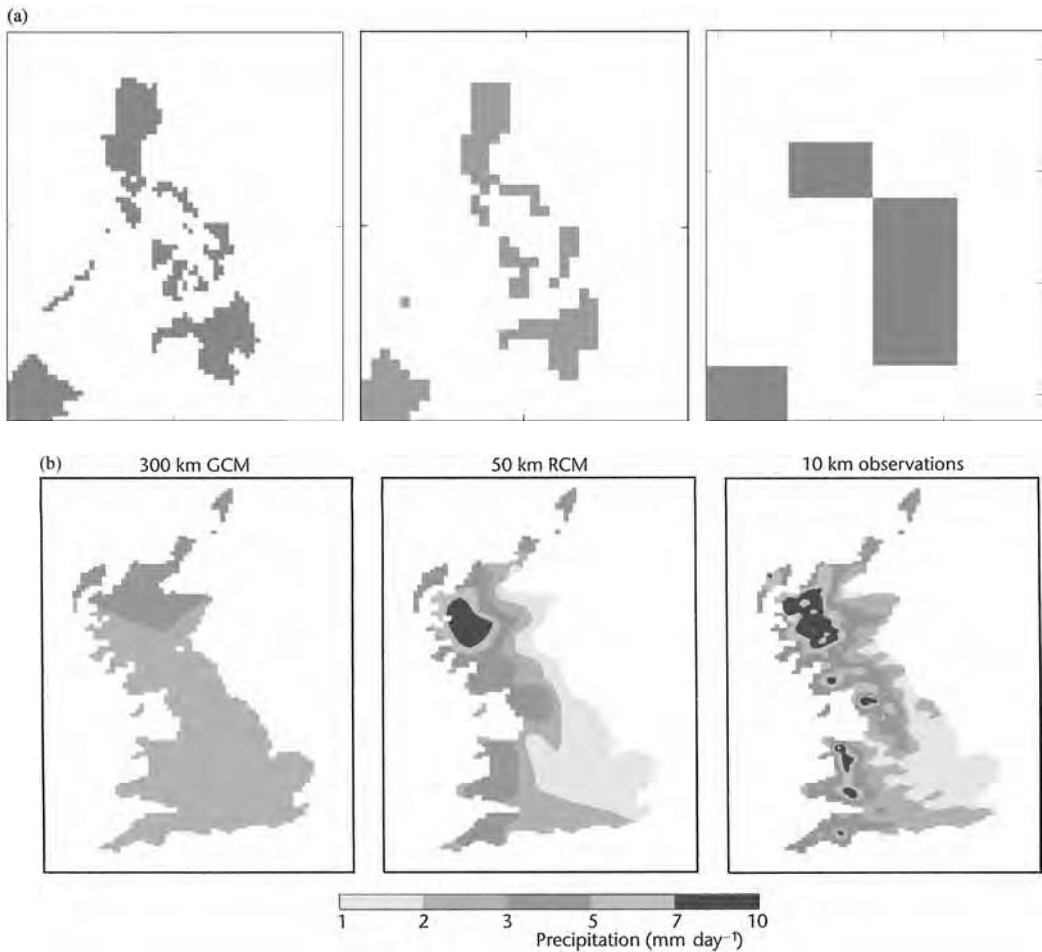
Figure 5.24 (a) Representation of the Philippines in RCMs with resolutions of 25 km and 50 km and in a GCM with 400 km resolution; (b) patterns of present-day winter precipitation over Great Britain, (i) as simulated with a 300 km resolution global model, (ii) with 50 km resolution regional model, (iii) as observed with 10 km resolution.
