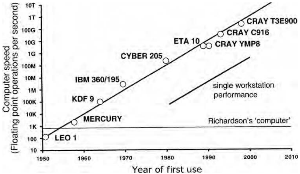
Figure 5.1 Illustrating the growth of computer power available at major forecasting centres. The computers are those used by the UK Meteorological Office for numerical weather prediction research, since 1965 for operational weather forecasting and most recently for research into climate prediction. Richardson's computer refers to his dream of a large 'human' computer mentioned at the beginning of the chapter.
