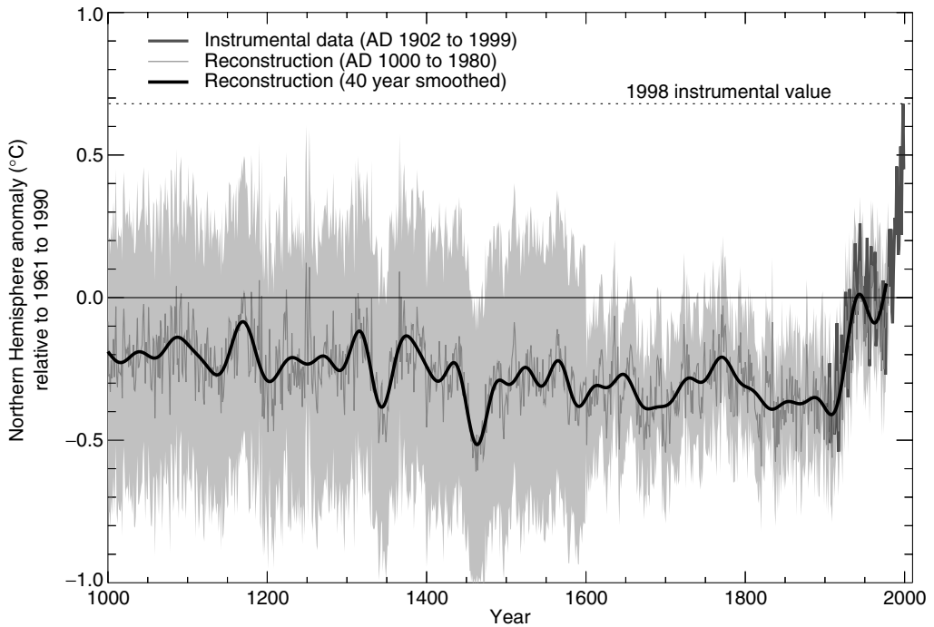
Figure 4.3 Millennial Northern Hemisphere temperature reconstruction from tree rings, corals, ice cores and historical records (for the period 1000–1980) and from instrumental data (for 1902–1999). A smoothed version of the proxy record is also shown, as are the 95% confidence limits (grey shaded).
