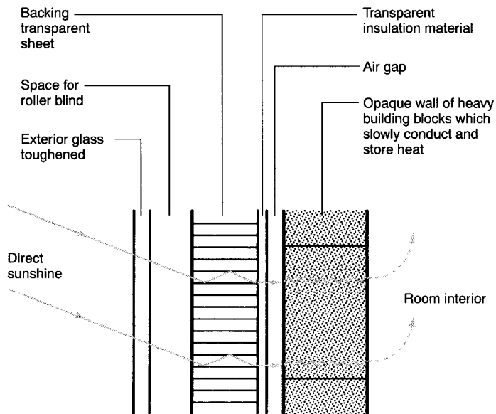
Figure 11.12 Construction of a 'solar wall'. The insulation material is about 100 mm thick and consists of open honeycomb channels of transparent polycarbonate material.
